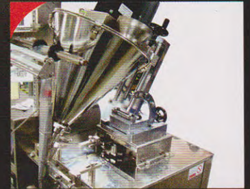
Screw Auger System
